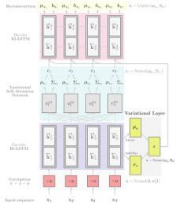
Fig. 1. Variational Bi-LSTM Autoencoder with Variational Self-Attention.
